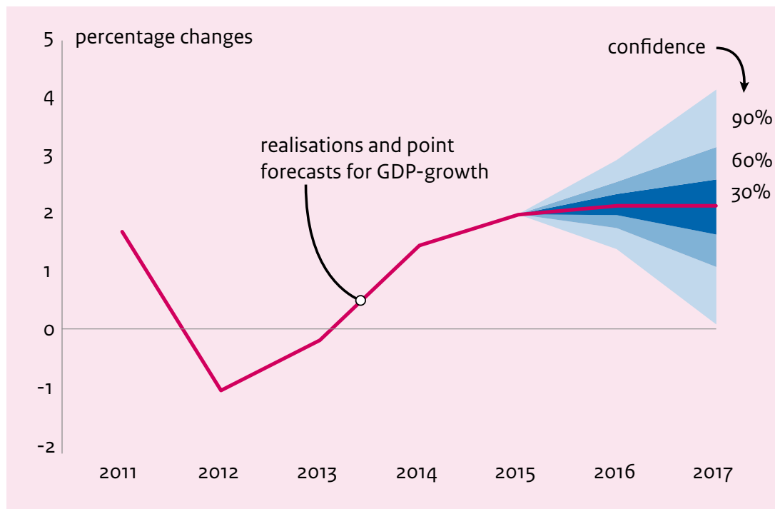
Figure 1 GDP-growth
